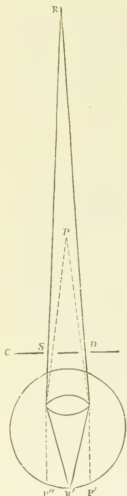
Fig. 180.—Scheiner's Experiment.
